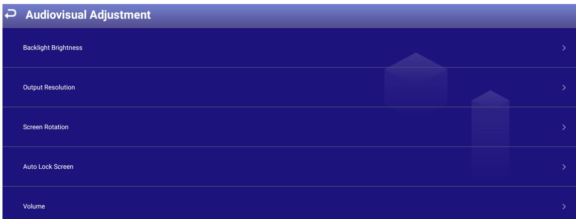
Figure 5-3 Audiovisual adjustment
