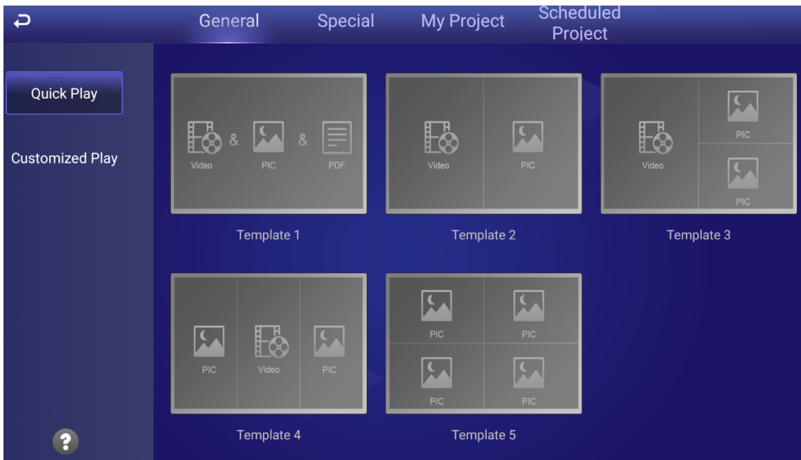
Figure 4-16 Quick play
