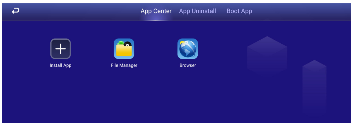
Figure 4-27 App center
