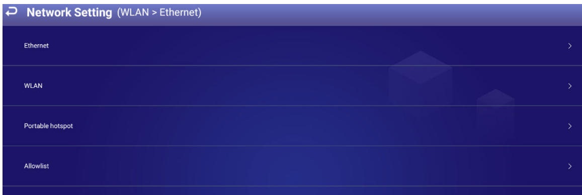
Figure 4-10 Network setting
