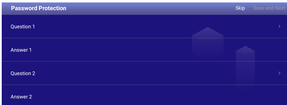
Figure 4-2 Password protection
