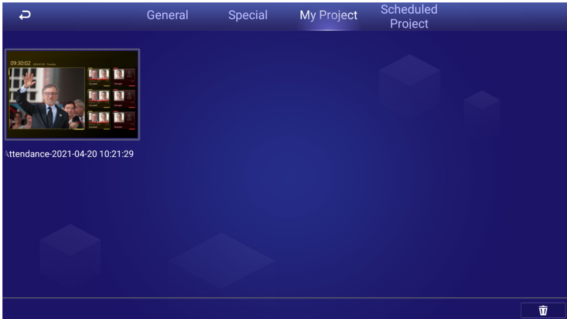
Figure 4-23 My project
