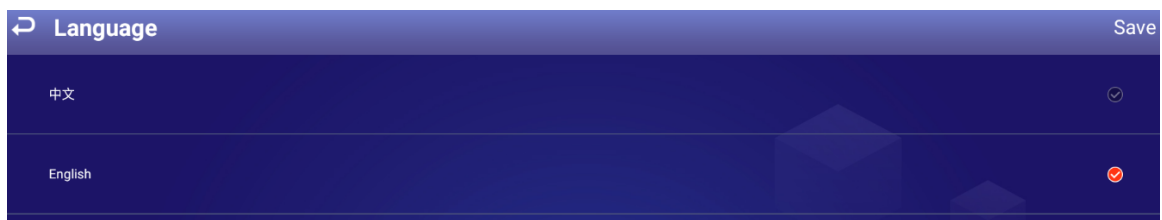
Figure 5-4 Language
