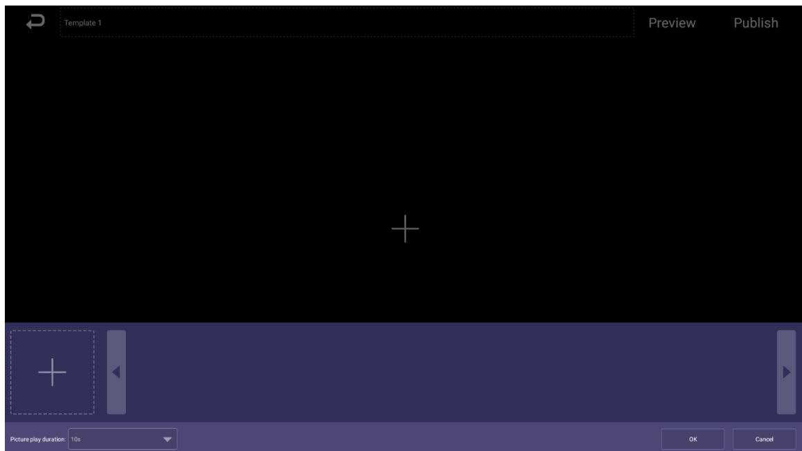
Figure 4-18 Add media
