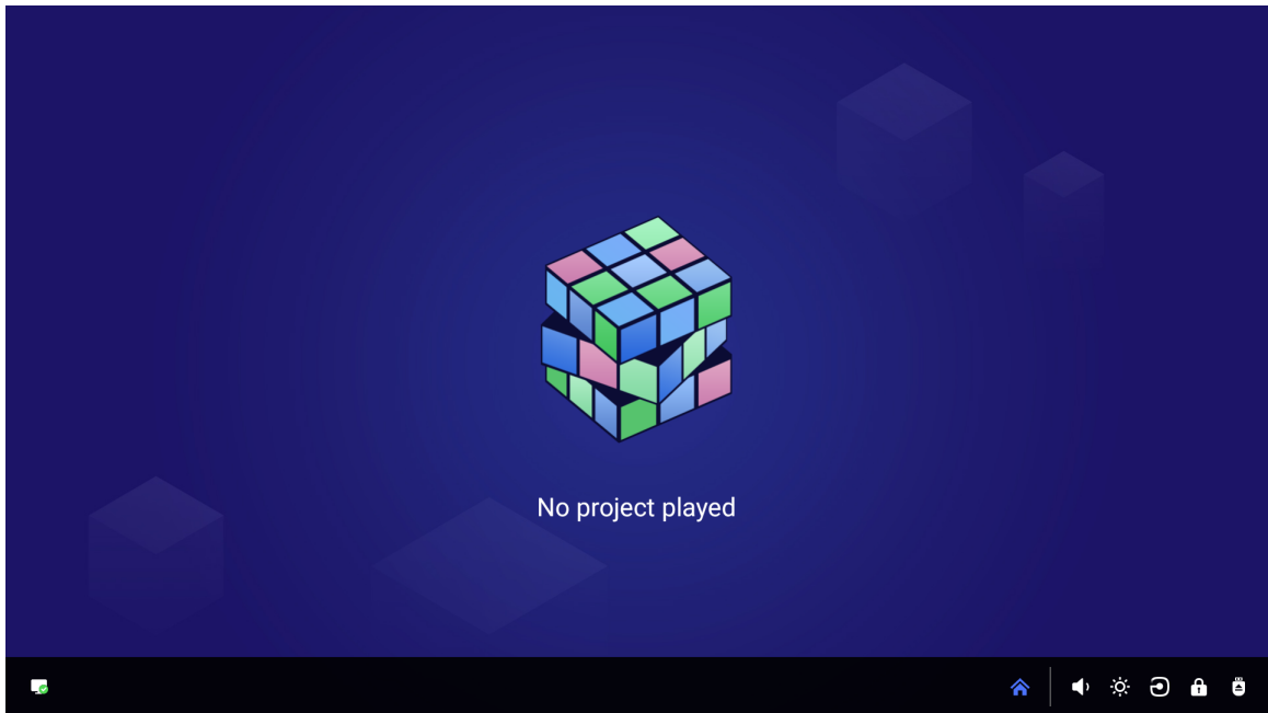
Figure 4-12 Network release
