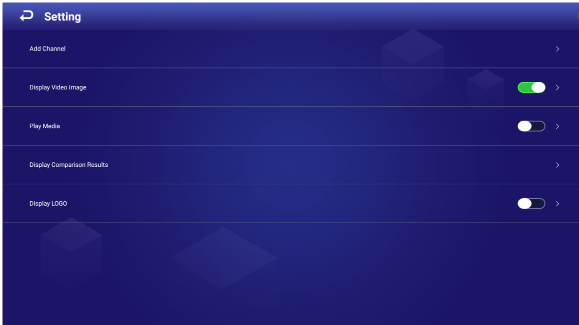
Figure 4-20 Setting
