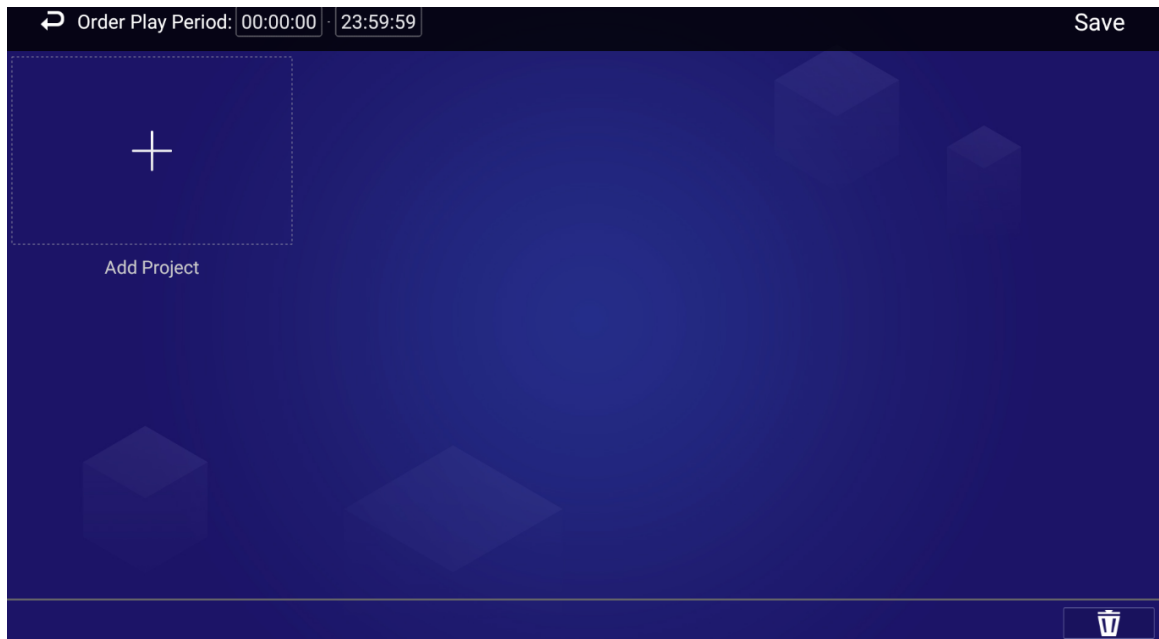
Figure 4-26 Add project
